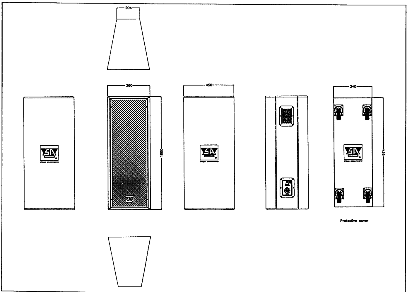
Physical dimensions of the SA 4826; normal version. The protective cover/dolly for transportation is shown at the right side.
