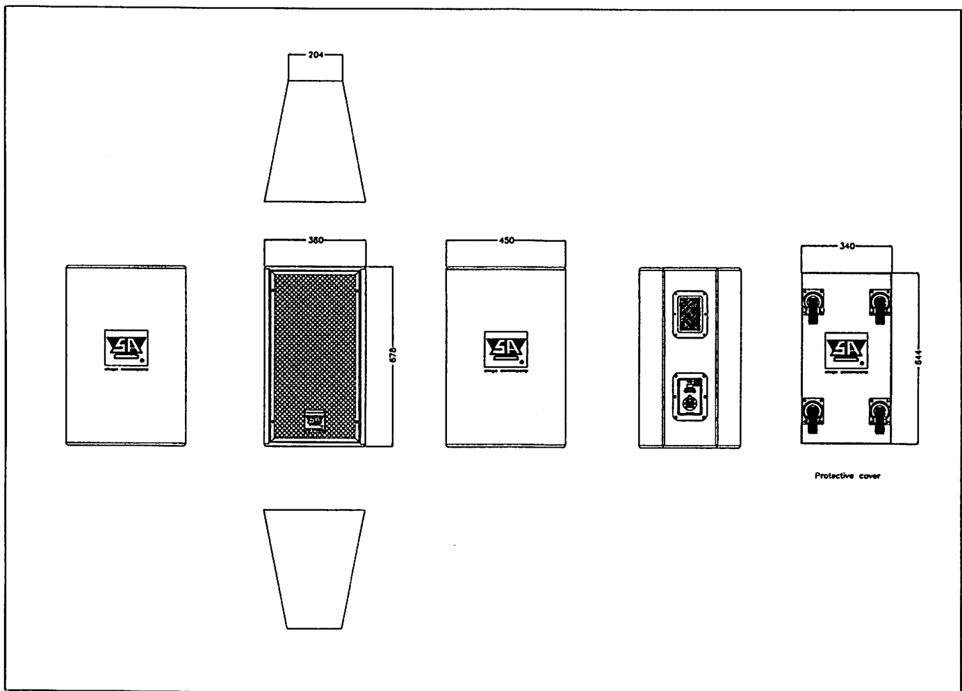
Physical dimensions of the SA 4824; normal version. The protective cover/dolly for transportation is shown at the right side.
