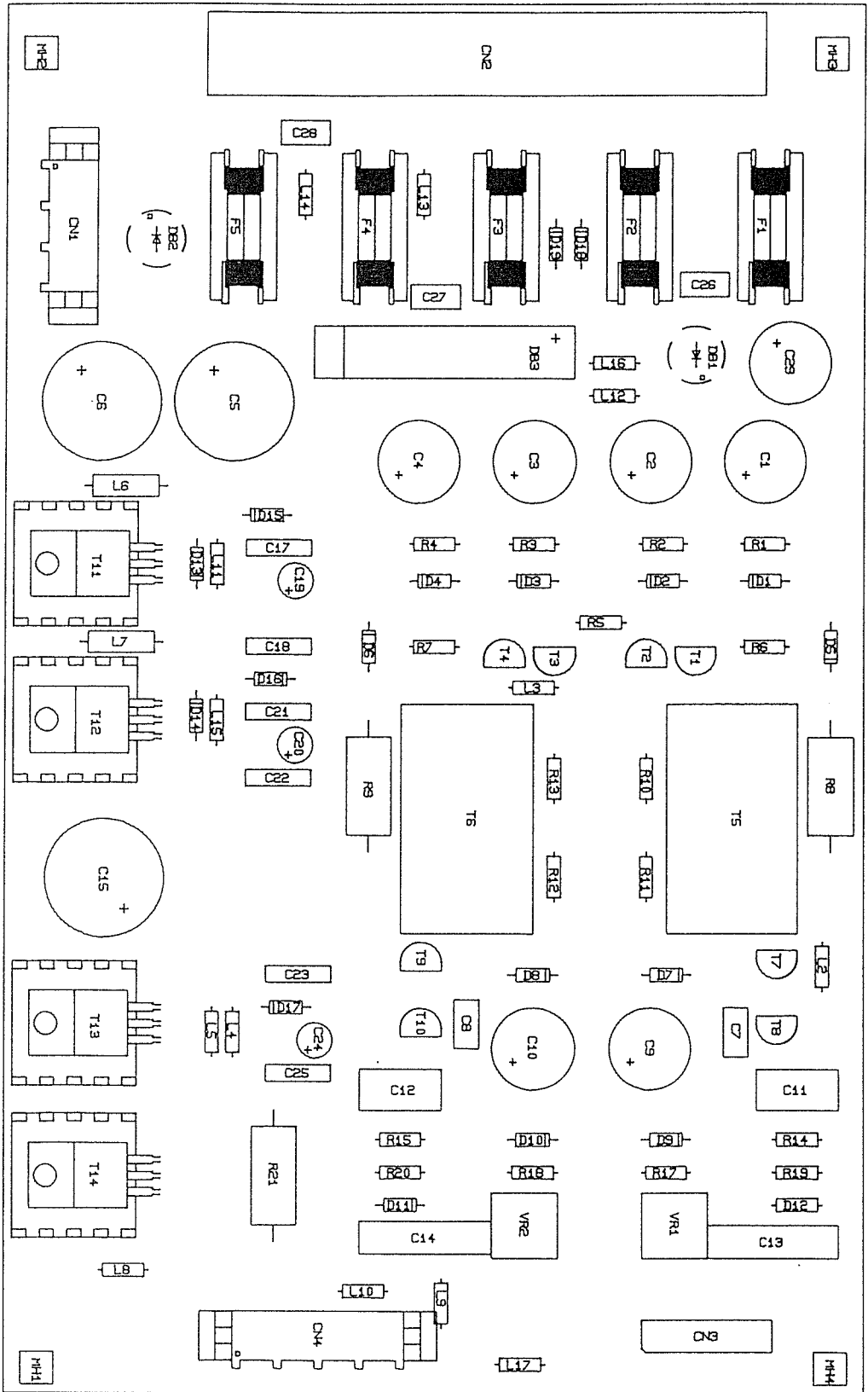
regulated power supply board
